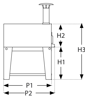
Vista laterale - View from the side
