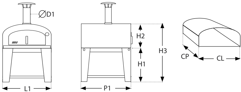
Vista frontale - View from the front Vista laterale - View from the side Camera di cottura - Cooking chamber
